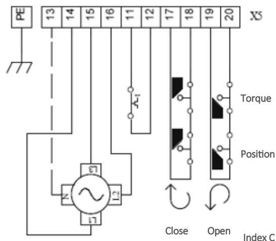
3-Phase AC
