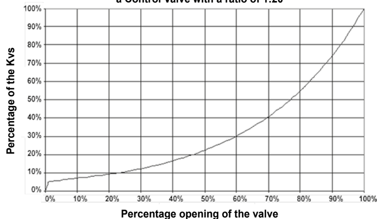
Equal percentage characteristic of a Control Valve with a ratio of 1:20
